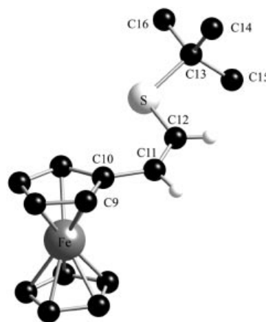
Figure 3. Ball-and-stick view of the molecular structure of 4b showing the (Z) configuration around the \text{C}=\text{C} bond. For clarity, only the vinylic hydrogen atoms are shown. Selected bond lengths [Å] and angles ^\circ : \text{C}(10)\text{--}\text{C}(11) 1.458(7), \text{C}(11)\text{--}\text{C}(12) 1.351(8), \text{C}(12)\text{--}\text{S} 1.749(5), \text{C}(13)\text{--}\text{S} 1.845(5), \text{C}(13)\text{--}\text{C}(14) 1.545(7); \text{C}(9)\text{--}\text{C}(10)\text{--}\text{C}(11) 123.1(5), \text{C}(10)\text{--}\text{C}(11)\text{--}\text{C}(12) 128.8(5), \text{C}(11)\text{--}\text{C}(12)\text{--}\text{S} 125.0(4), \text{C}(12)\text{--}\text{S}\text{--}\text{C}(13) 103.0(3), \text{C}(14)\text{--}\text{C}(13)\text{--}\text{S} 110.1(3), \text{C}(15)\text{--}\text{C}(13)\text{--}\text{S} 110.8(4), \text{C}(16)\text{--}\text{C}(13)\text{--}\text{S} 103.5(4).
