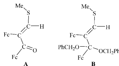
Figure 3. Ball-and-stick view of the molecular structure of 4b showing the (Z) configuration around the \text{C}=\text{C} bond. For clarity, only the vinylic hydrogen atoms are shown. Selected bond lengths [Å] and angles ^\circ : \text{C}(10)\text{--}\text{C}(11) 1.458(7), \text{C}(11)\text{--}\text{C}(12) 1.351(8), \text{C}(12)\text{--}\text{S} 1.749(5), \text{C}(13)\text{--}\text{S} 1.845(5), \text{C}(13)\text{--}\text{C}(14) 1.545(7); \text{C}(9)\text{--}\text{C}(10)\text{--}\text{C}(11) 123.1(5), \text{C}(10)\text{--}\text{C}(11)\text{--}\text{C}(12) 128.8(5), \text{C}(11)\text{--}\text{C}(12)\text{--}\text{S} 125.0(4), \text{C}(12)\text{--}\text{S}\text{--}\text{C}(13) 103.0(3), \text{C}(14)\text{--}\text{C}(13)\text{--}\text{S} 110.1(3), \text{C}(15)\text{--}\text{C}(13)\text{--}\text{S} 110.8(4), \text{C}(16)\text{--}\text{C}(13)\text{--}\text{S} 103.5(4).
